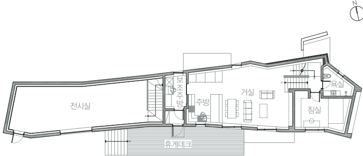
PLAN - 2F (178.10m 2 )
